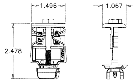
MULTI-CLAMP 6000 SERIES ALUMINUM (Fy MIN. = 35.0 KSI) (Fu MIN. = 38.0 KSI)
