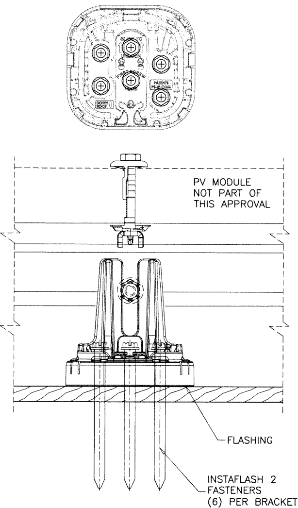
SECTION C-C
