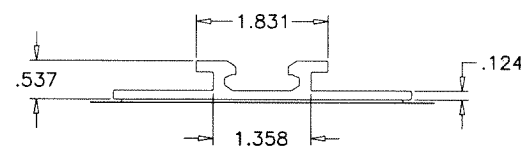
SCISSOR MOUNT ASSEMBLY 6000 SERIES ALUMINUM (Fy MIN. = 35.0 KSI) (Fu MIN. = 38.0 KSI)
