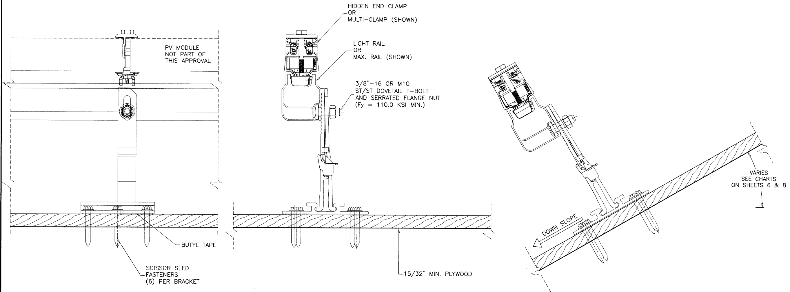
SECTION B-B
